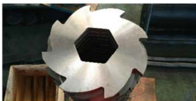
双轴撕碎机动刀 Double Shaft Shredder Blades
